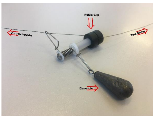
Auto-Lib Downrigger
